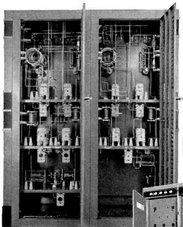
DOUBLE CUBICLE, 5 KW UNIT, rear view, showing the compact but uncrowded arrangement of components. Large rear doors are interlocked for safety, provide easy access for maintenance or adjustment.
